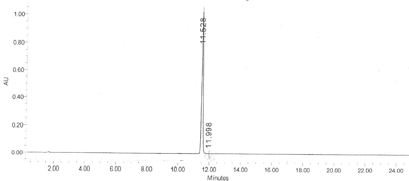
Auto-Scaled Chromatogram
